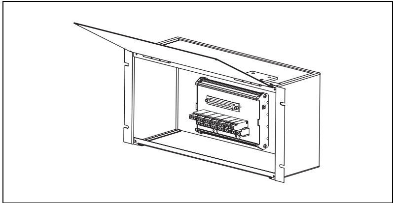
Figure 1. CB-37F-HVD and UL Listed Enclosure
